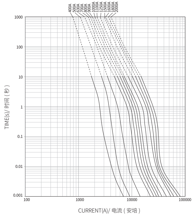
H4FG 平均 I-T 曲线图 (仅供参考) AVERAGE I-T CHARACTERISTICS CURVE (FOR REFERENCE ONLY)
